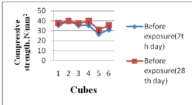
Fig.1. Compressive strength before exposure
