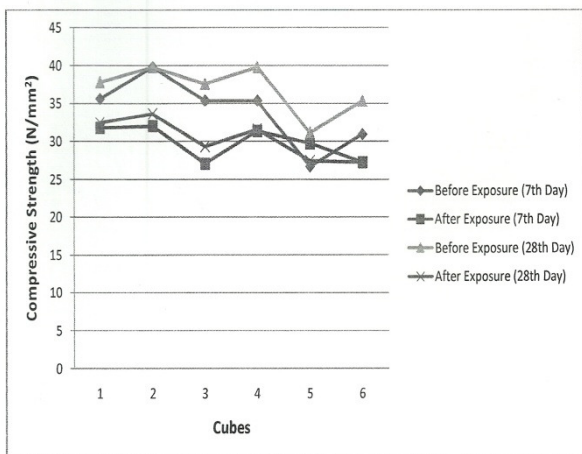
Fig.3. Change in compressive strength of concrete exposed to 5% sulfuric acid solution.
