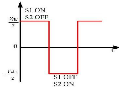
Figure 3.1.2: Inverter Output
