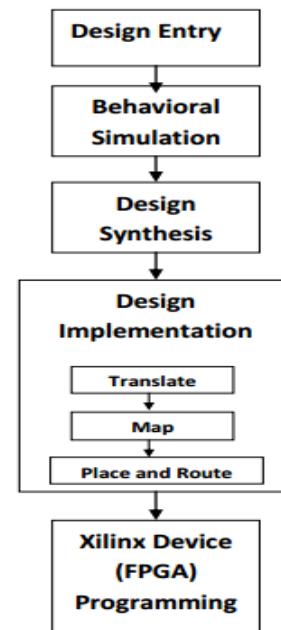
Figure 4.1 Design Flow
