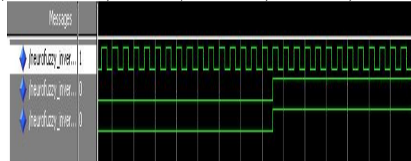
Figure 4.3.1: Simulation Output for D = 20%
