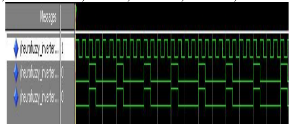
Figure 4.3.2: Simulation Output for D = 25%
