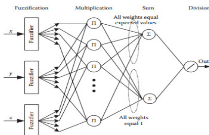
Figure 3.1.2: Neuro-Fuzzy System
