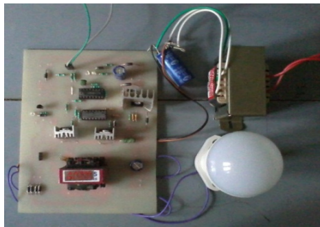
Figure 4.2.2: Design 1- \phi Voltage source half-bridge MOSFET based PWM Inverter
