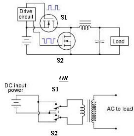
Figure 3.1.1: Circuit Schematic
