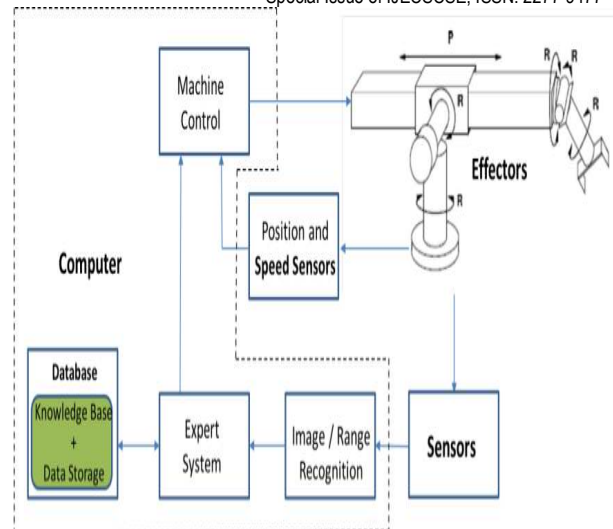
Figure 1. Components of an Intelligent Robot
